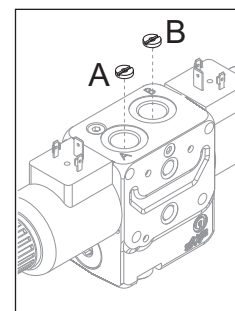
Interchangeable holed washer into fittings ports
