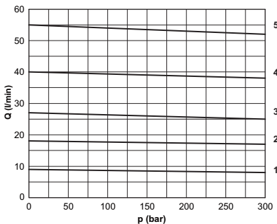
Compensation curves
