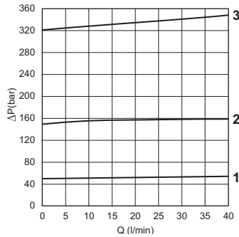
PRESSURE-FLOW RATE
